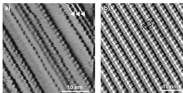
Figure 5. STM images of the network generated upon combining tecton 6 with a) \text{CoCl}_2 and b) \text{Pd}^{\text{II}} . Image (a) shows the formation of laterally uncorrelated 1D nanostructures, while (b) displays the parallel packing of 1D networks that leads to the generation of a 2D nanoscale array. a) V_{\text{tip}} = 705 mV; I_t = 13 pA; b) V_{\text{tip}} = 983 mV; I_t = 13.6 pA.
